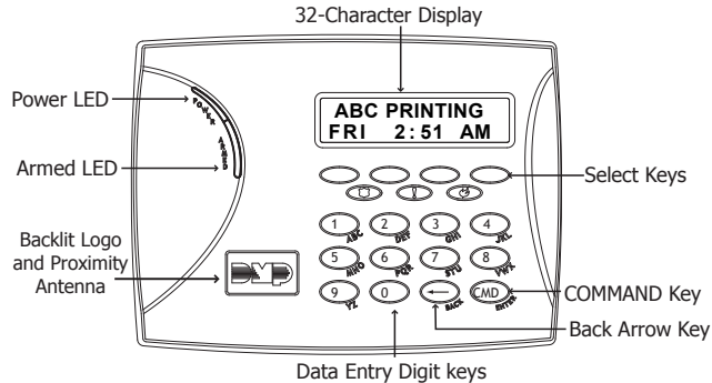
Thinline™/Aqualite™ Keypad
